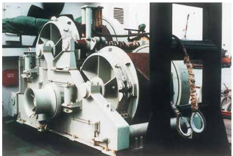
DIESEL ENGINE DRIVEN ANCHOR HANDLING & TOWING WINCH
